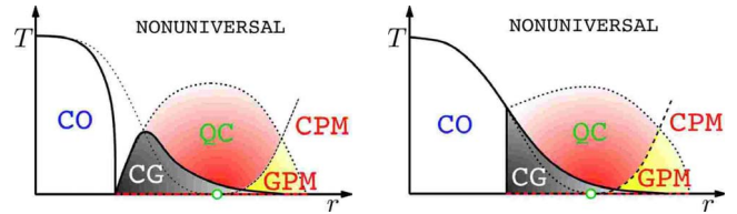
FIG. 2. (Color online) Schematic phase diagrams of a disordered itinerant quantum antiferromagnet close to the quantum phase transition showing two possible scenarios for the appearance of a cluster glass phase, which is denoted by CG. The other labels are as in Fig. 1.
